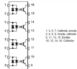
* U11~U12 Pin Configuration
